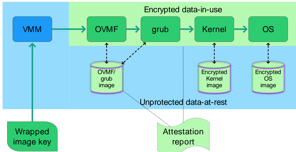
FIGURE 28: MEASURED START WITH FULLY ENCRYPTED DISK IMAGES
